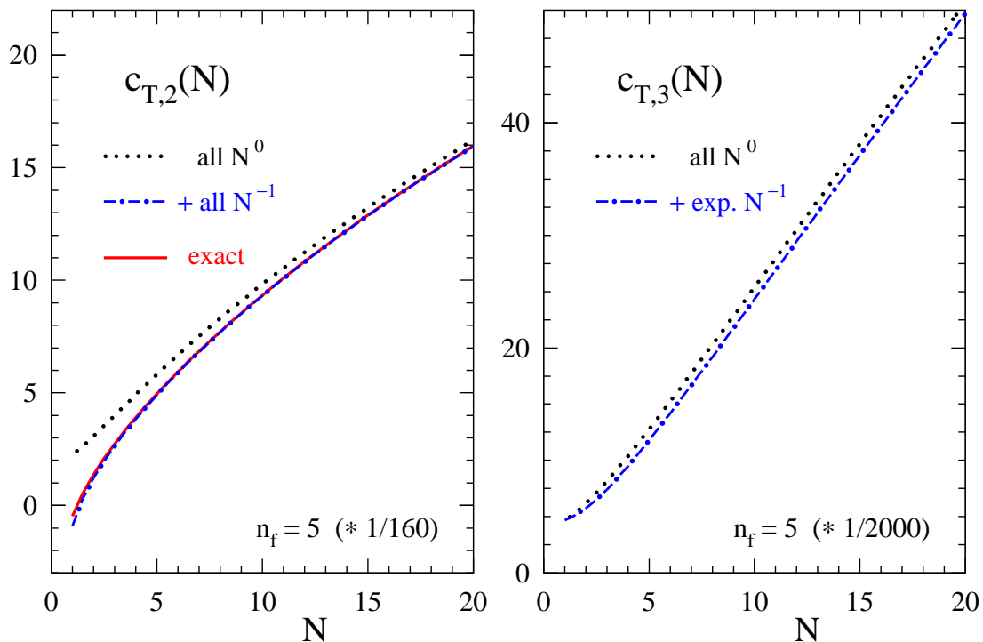
Figure 2. As figure 1, but for the fragmentation function F_T at n_f = 5 . Neither the exact three-loop result nor the corresponding coefficients of the N^{-1} \ln N and N^{-1} terms are known at present.
