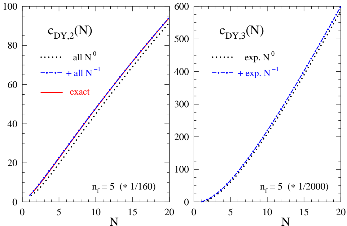
Figure 4. As figure 2, but for Drell-Yan cross section (2.11), using the expansions (7.7) and (7.8) with \xi_{\text{DY}_3} = -400 . Besides the coefficients mentioned in the caption of that figure, also the third-order constant- N and N^{-1} \ln^2 N coefficient are unknown in this case.
